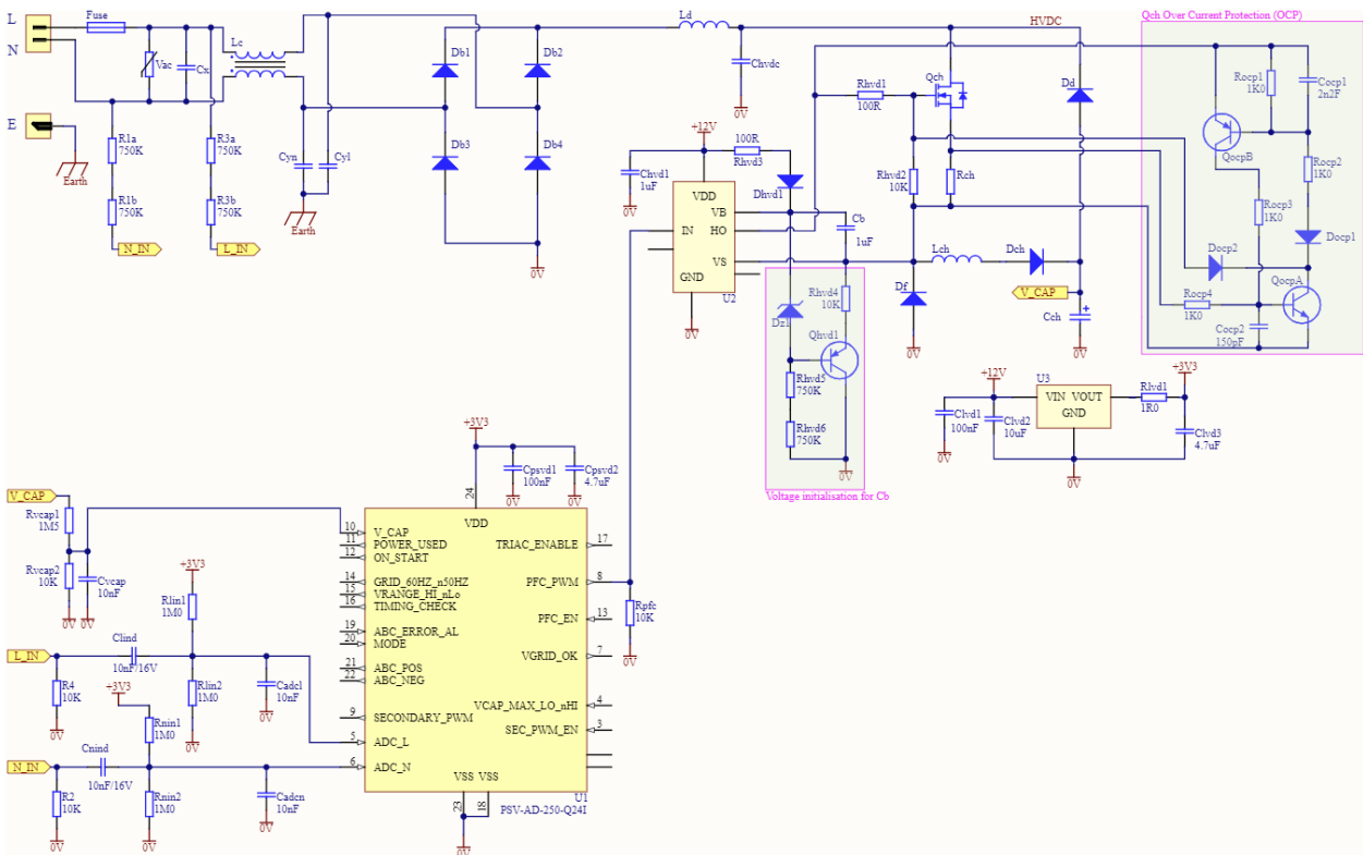
Figure 1f: PSV-AD-xxx Controller Basic Functional Schematic
