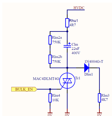
Figure 2.4a - External Components for the PSV-AD-xxx-DS to Provide System Holdup
