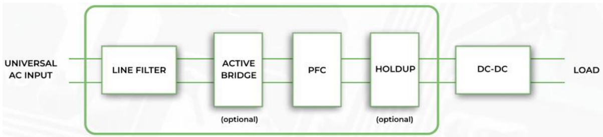
Figure 1e: PSV-AD-xxx-DS System Block Diagram
