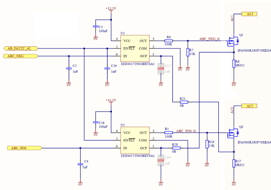
Figure 2.5a - PSV-AD-xxx-DS Active Bridge Circuit
